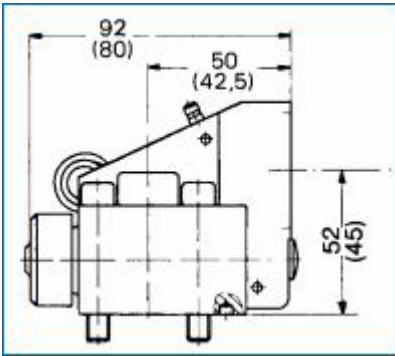
Valve body with console
